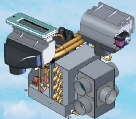
SPLITAIR UNITS 5000 to 20000 BTU
