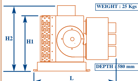
FRESHAIR48 - FRESH-AIR 48000 BTU - LAT. VIEW
