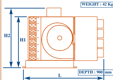
EXTRACT24 - AIR EXTRACTION UNIT - LAT. VIEW
